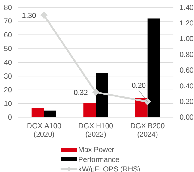
Chart 5: Improvement in hardware efficiency (NVIDIA Corporation, 2024)
